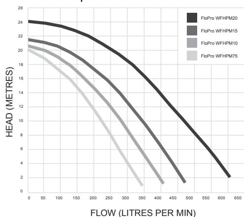
Pump Performance Curve
